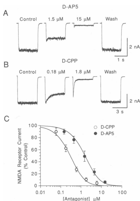
FIGURE 4 Equilibrium dose-response data for competitive NMDA receptor antagonists analyzed with a two binding site model. A shows responses to concentration jump application of 10 \mu M NMDA, applied together with the indicated concentrations of D-AP5; 3 \mu M glycine was present continuously. The activation of NMDA receptors by agonist and the onset of antagonism by D-AP5 reach equilibrium with similar kinetics. B shows similar responses, in a different neuron, for D-CPP. Initially, the response to NMDA overshoots its equilibrium value, because the onset of antagonism by D-CPP is slow to reach equilibrium. C shows the equilibrium dose response curve for block of the response to NMDA by D-AP5 and D-CPP; data points are the mean \pm S.D. of values recorded from four neurons per antagonist. The solid line drawn through the data points was obtained by a least squares fit of Eq. 8, the equilibrium equation for a two binding site model.
