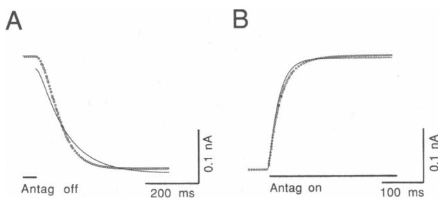
FIGURE 3 Analysis of two-site simulated responses by a one-site model. The response to a concentration jump application of antagonist was simulated by a two-site model for antagonist action (small circles) and analyzed using a one-site model for antagonist action (solid line). A shows recovery from antagonism, B the onset of antagonism. Values for agonist and antagonist binding kinetics were chosen such that they approximated the experimental values obtained with NMDA and D-AP5. Parameters for two-site model simulation were: k_{Aon} = 2 \mu\text{M}^{-1}\text{s}^{-1} , k_{Aoff} = 23 \text{ s}^{-1} , k_{Bon} = 16 \mu\text{M}^{-1}\text{s}^{-1} , k_{Boff} = 20 \text{ s}^{-1} , [A] = 10 \mu\text{M} agonist, [B] = 10 \mu\text{M} antagonist. To determine k_{Aon} and k_{Aoff} for the one-site model analysis, the response of the two-site model to agonist concentration jumps was simulated (not shown), and the results fit with single exponential functions. Agonist and antagonist association and dissociation rate constants obtained by one-site analysis of these simulated responses were: k_{Aon} = 1.2 \mu\text{M}^{-1}\text{s}^{-1} , k_{Aoff} = 46 \text{ s}^{-1} , k_{Bon} = 20.5 \mu\text{M}^{-1}\text{s}^{-1} , k_{Boff} = 9.9 \text{ s}^{-1} .
